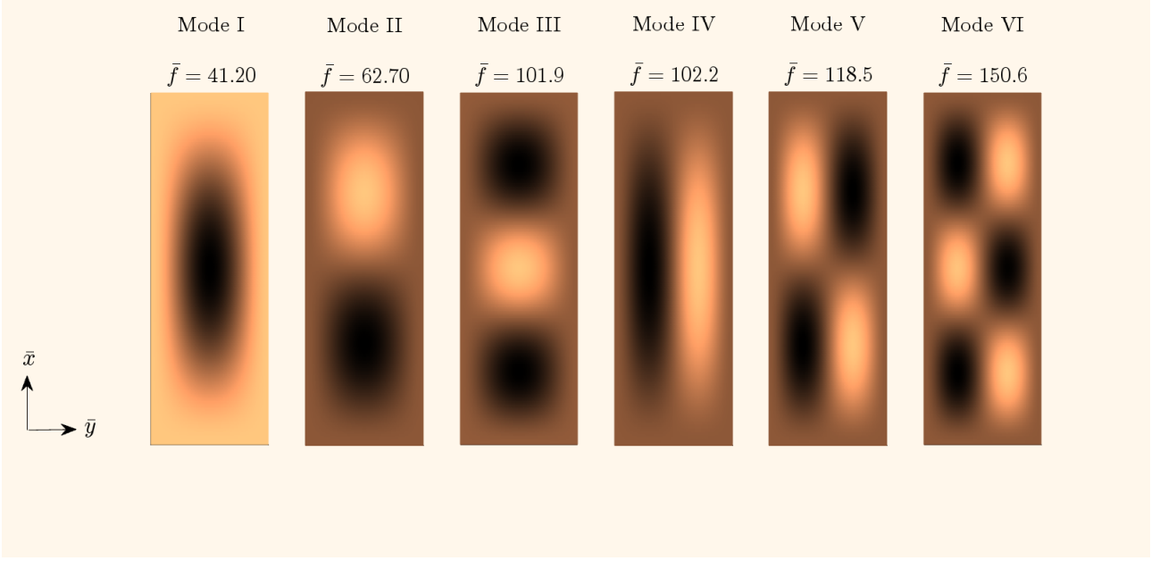
Figure 3: Nondimensional baseline modal shapes and frequencies. For visualisation purposes, the x axis is vertical in the figure. The frequencies are computed to their converged value up the fourth significant digit, as given. Note that the baseline mode shapes are identified through a Roman numeral.
